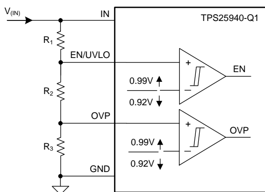
Figure 43. UVLO and OVP Thresholds Set By R_1 , R_2 and R_3
